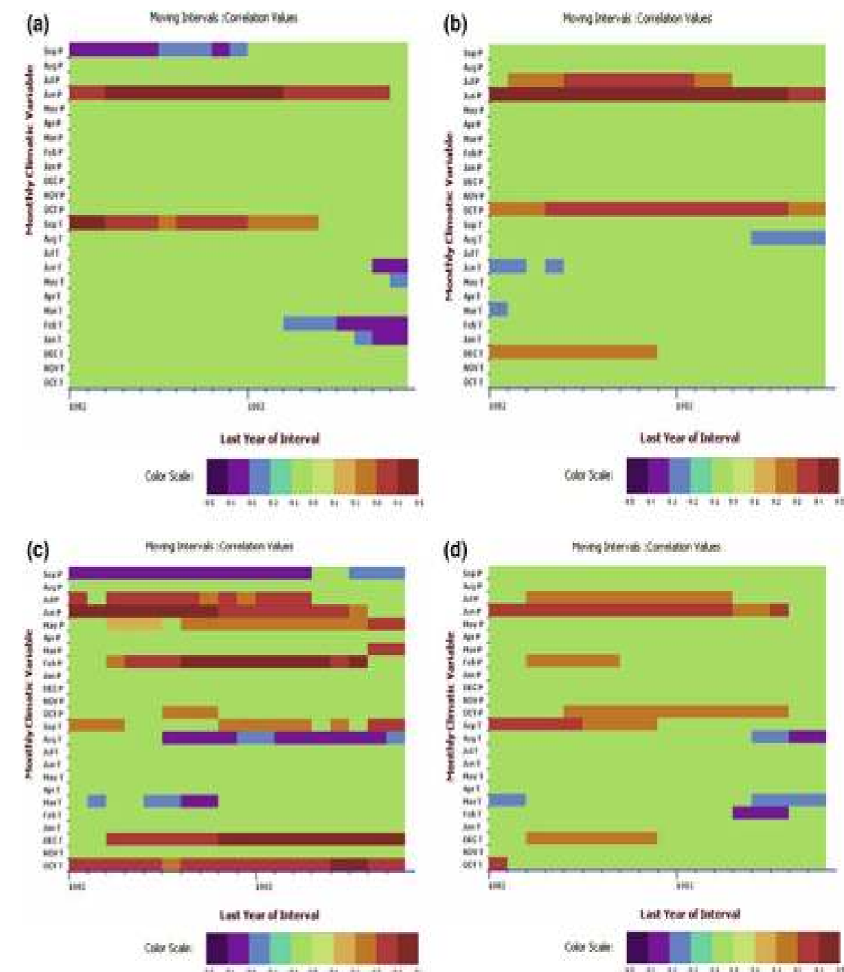
Fig. 3 Moving correlations between climate variables (monthly mean temperature (T) and monthly total precipitation (P)) and tree ring chronologies (a) S1; (b) S2; (c) PII; (d) PID;
