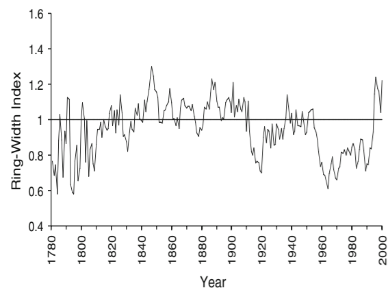
Fig. 5 Site chronology of Abies fargesii of the subalpine fir forest in the Qinling Mountains of Shaanxi province, China
