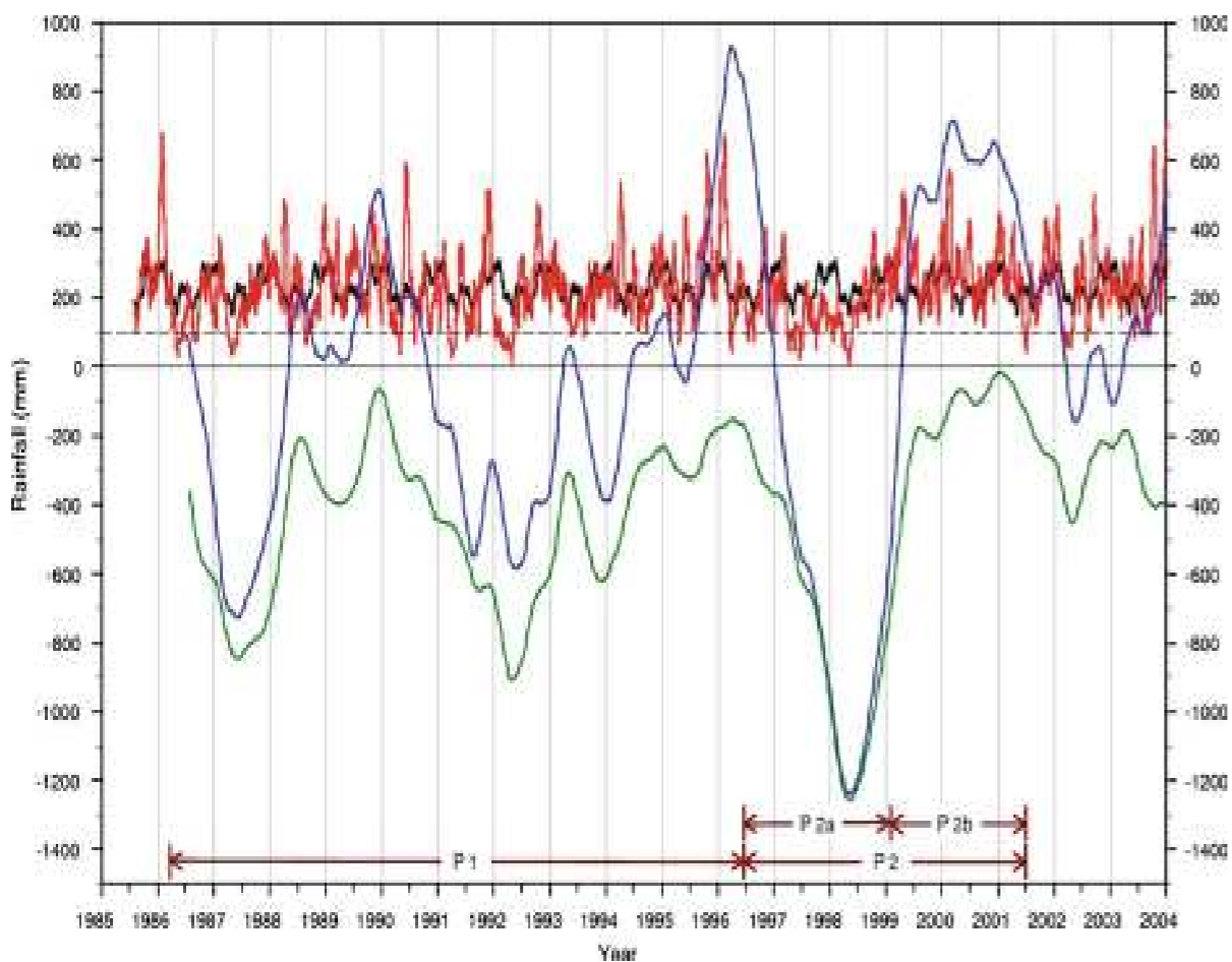
Fig. 1 Accumulated rainfall anomalies (ARA) with conditions applied at Danum, 1985–2003: R_{30} of mean daily (MDR; black line) and actual (ADR; red) rainfall, ARA_{365} (blue) and accumulation only when R_{30} < 232 mm ( CARA_{232} ; dark green); dashed reference at 100 mm (see text for explanations). Smoothing algorithm used a negative exponential function with
