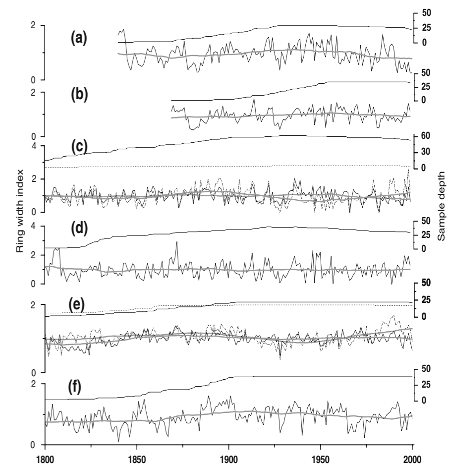
Fig. 2 The standard ring-width chronologies, 48-year smoothing (thicker line), and their corresponding sample depth, (a) S1; (b) S2; (c) P1, dashed line P1I and continuous line P1D; (d) P2; (e) J1, dashed line J1I and continuous line J1D; (f) J2
